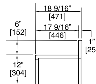
End View TS6FA
