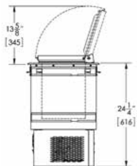
End view drop-in ice cream unit
