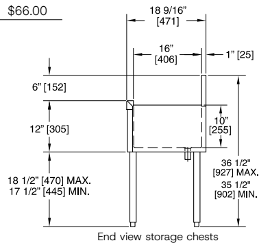
End view storage chests
