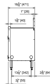
End view storage cabinet with sink
