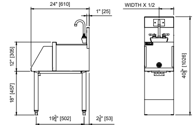
End view blender station with sink
