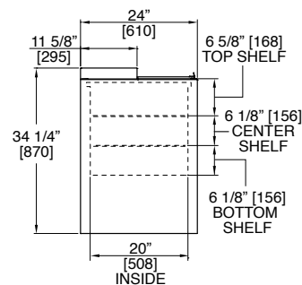
End view for 2' model
