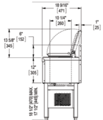
End view ice cream cabinet
