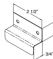
57420 (Millwork panel clip)
