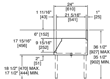
End view drop down drainboard
