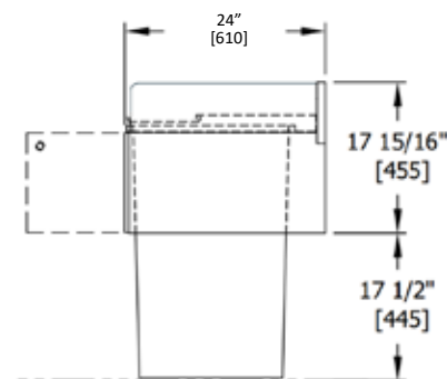
End view trash receptacle
