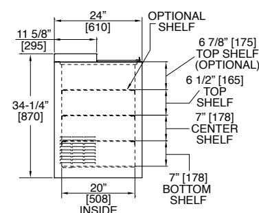
End view for 3', 4', &amp; 5' models
