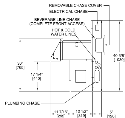
PEDESTAL BASE END VIEW
