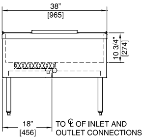
End view of service station ice chest
