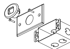
MBS-LED-CW (LED light, junction box, and cover)
