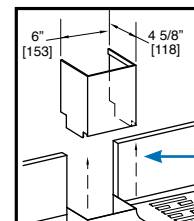
TS6CO-BW (with 7055-66 backsplash chase)
