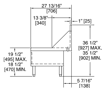
End view equipment stand
