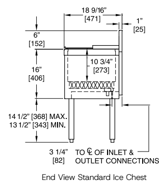
TS30IC10 Shown with cover and optional soda chase cutout
