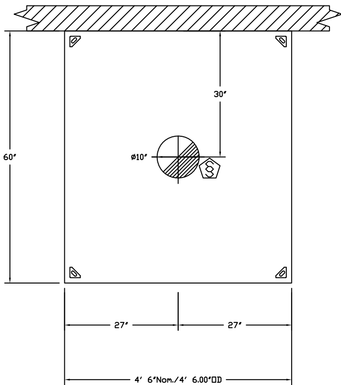
PLAN VIEW - Hood #1 (58) 4' 6.00" LONG 6024VHB
