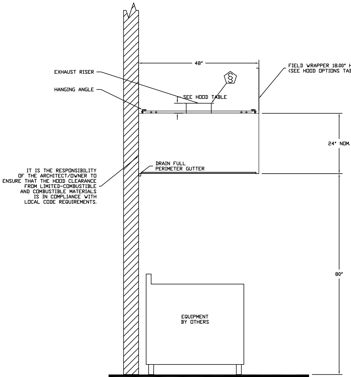
SECTION VIEW - MODEL 4824VHB-G HOOD - #2 (45)
