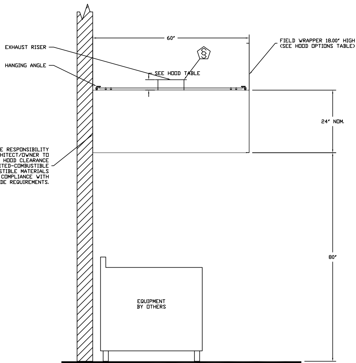
SECTION VIEW - MODEL 6024VHB HOOD - #1 (58)
