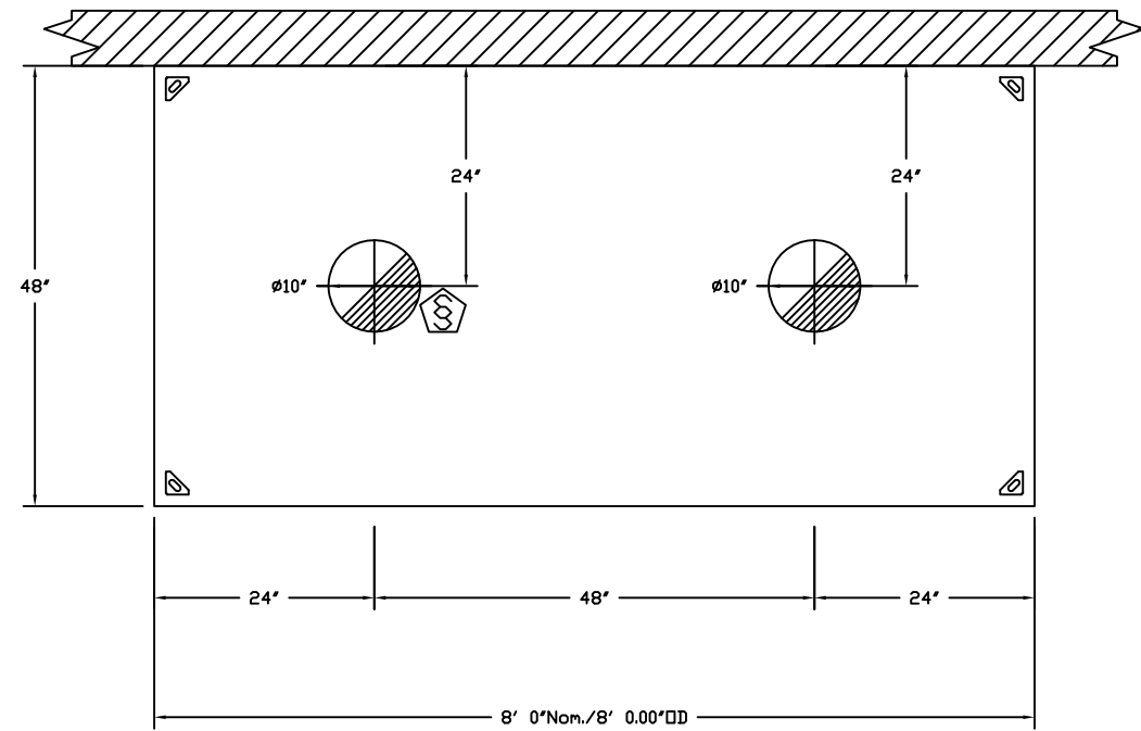
PLAN VIEW - Hood #2 (45) 8' 0.00" LONG 4824VHB-G
