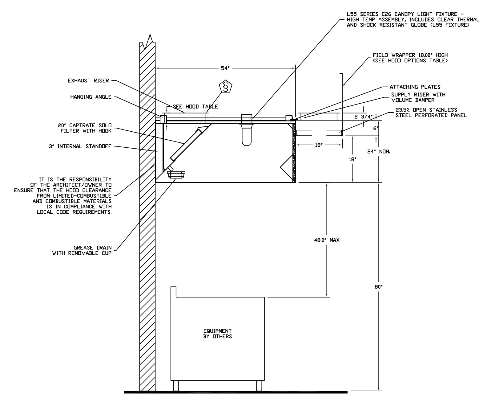
SECTION VIEW - MODEL 5424ND-2-PSP-F HOOD - #4 (1)
