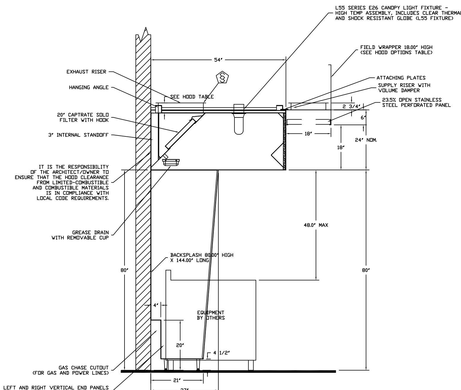
SECTION VIEW - MODEL 5424ND-2-PSP-F HOOD - #5 (155)
