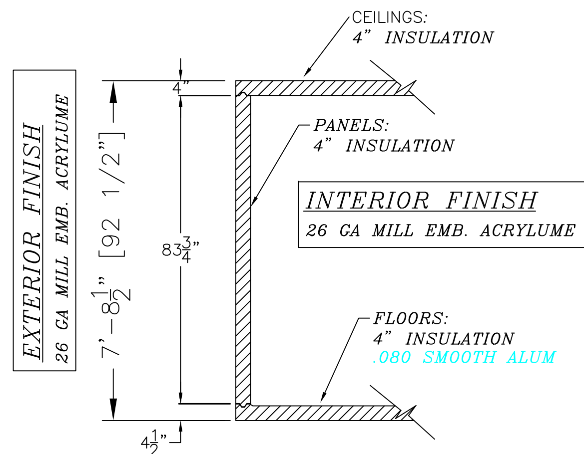
SECTION WALL WITH FLOOR
