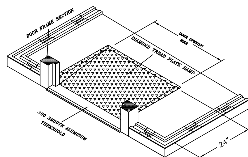
INTERIOR RAMP. STD ISOMETRIC VIEW
