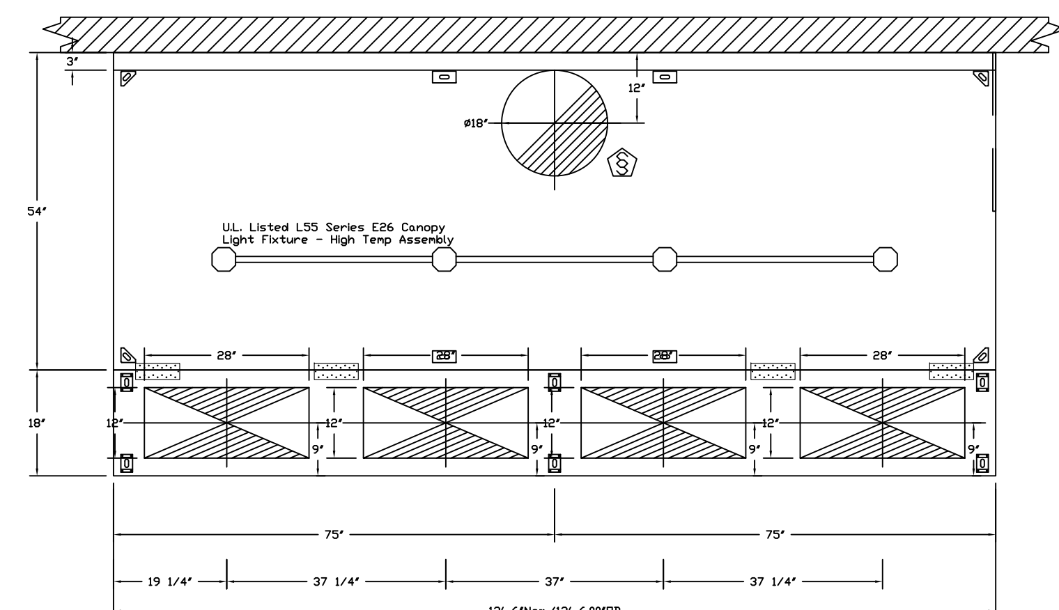
PLAN VIEW - Hood #5 (155) 12' 6.00' LONG 5424ND-2-PSP-F NOTE: Additional hanging angles provided for hoods 12' and longer.
